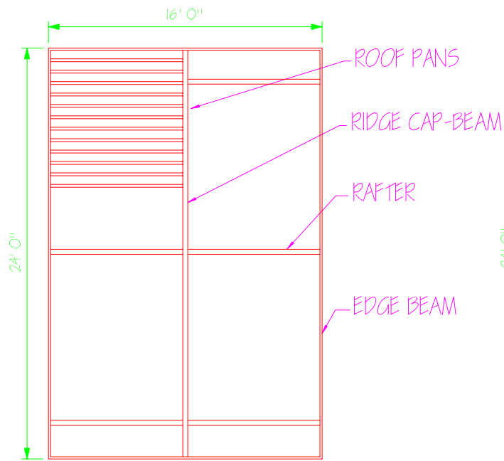
16x24 ILLINI SHELTER PLAN VIEW
