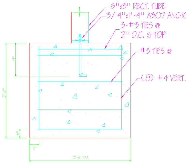
TYPICAL FOOTING
