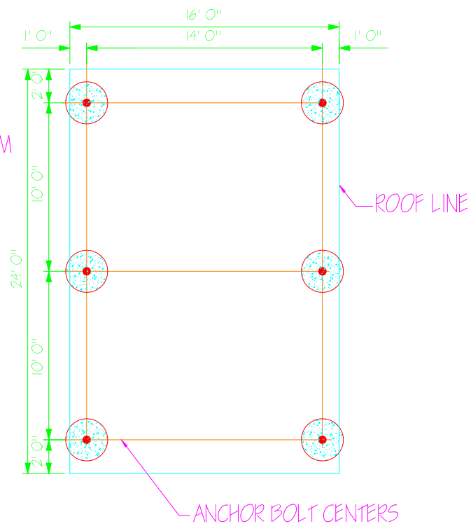
16x24 ILLINI SHELTER ANCHOR BOLT LOCATIONS PLAN VIEW
