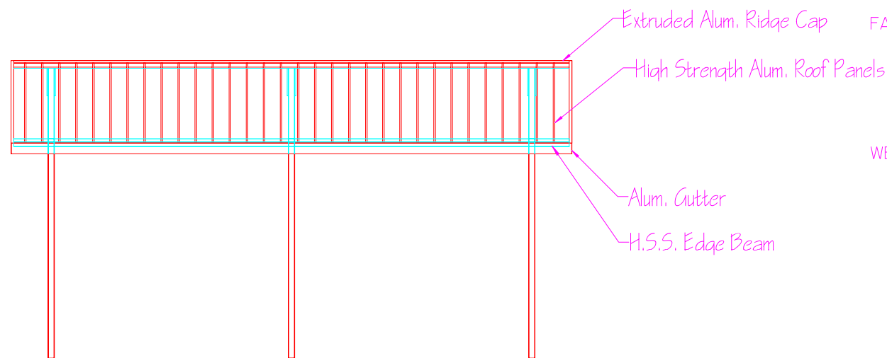
16x24 ILLINI SHELTER WEST ELEVATION
